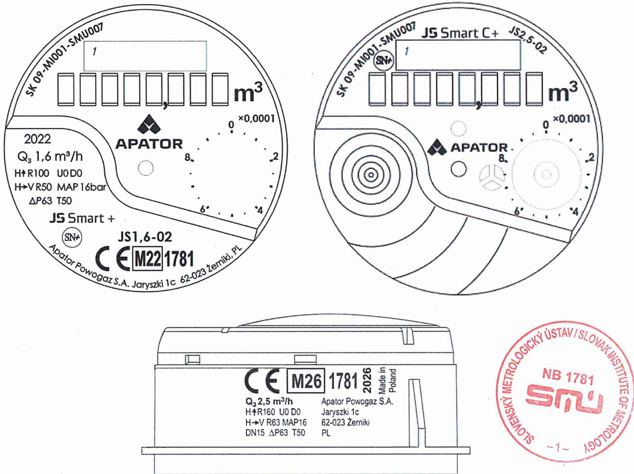
Picture No.2 Example of the dial marking
