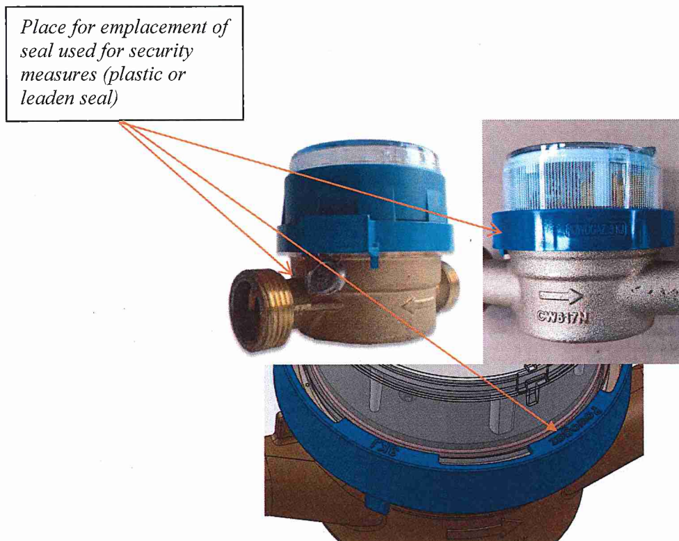
Picture No. 3 Emplacement of the seal used for security measures
